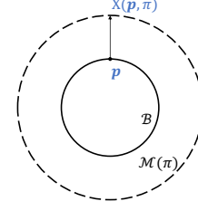
Figure 3: \chi(\mathbf{p}, \pi) is the intersection of \mathbf{p} 's normal with the evolving surface \mathcal{M}(\pi) .
