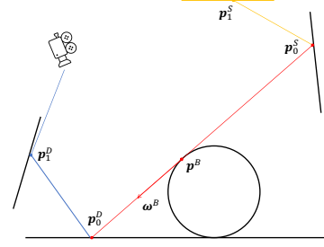
Figure 2: Boundary segments: A boundary light path (6) is comprised of a boundary segment (7) \overline{p_0^S p_0^D} (shown in red) as well as a source subpath (illustrated in orange and blue, respectively). The two endpoints of the boundary segment (7) are located on the visibility boundary of each other. A boundary segment (6) \overline{p_0^S p_0^D} can be uniquely determined with a surface point p^B \in \mathcal{B} interior to the segment, along with a direction \omega^B .
