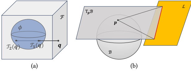
Figure 7: (a) We sample points from the implicit surface \phi by sampling a point q from the proxy \mathcal{F} and project q onto the implicit surface \phi . We then take all the intersections, \mathcal{T}_1(q) and \mathcal{T}_2(q) in this example, as the sample points from the implicit surface \phi . (b) We intersect the tangent plane T_p\mathcal{B} at p with light \mathcal{L} and only sample from tangent directions intersecting the light \mathcal{L}
